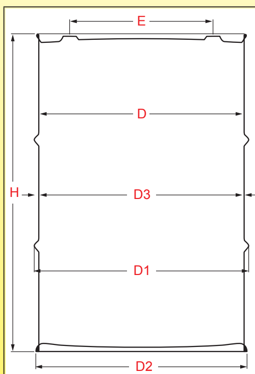
Usual dimensions of steel drums
