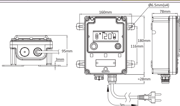
Model with 5 ways waterproof connector
