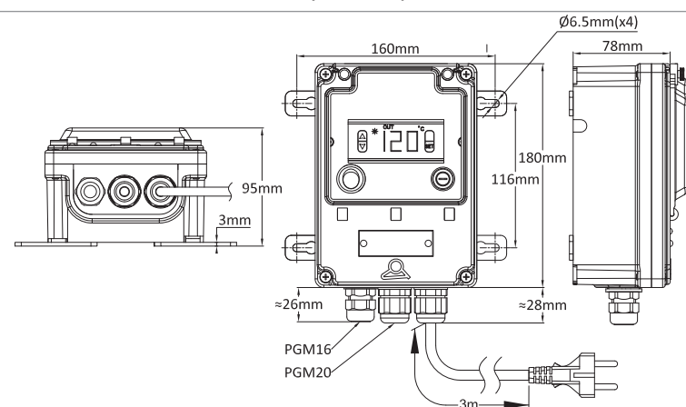
Model with 3 cable glands
